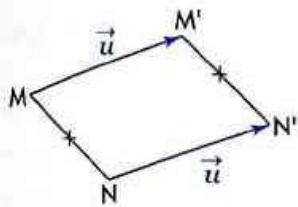
translation t_{\vec{u}} .
